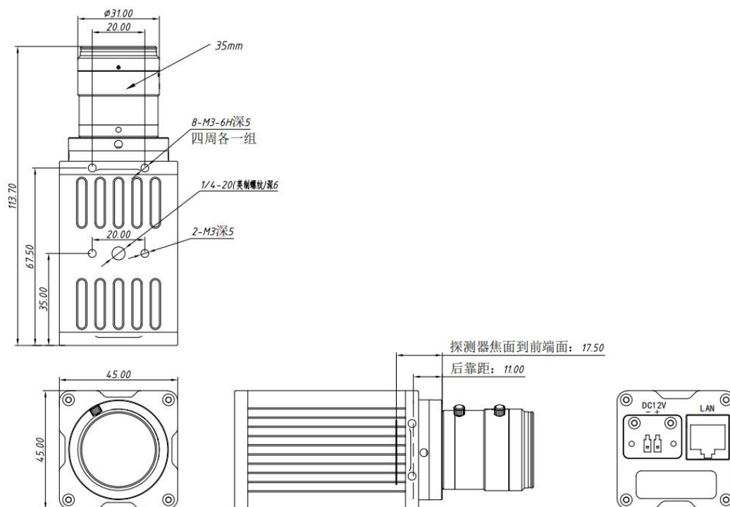
Figure 3 Structural dimensions
