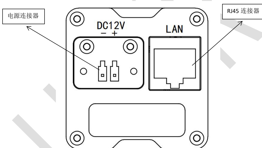
Figure 2 Interface Definition
