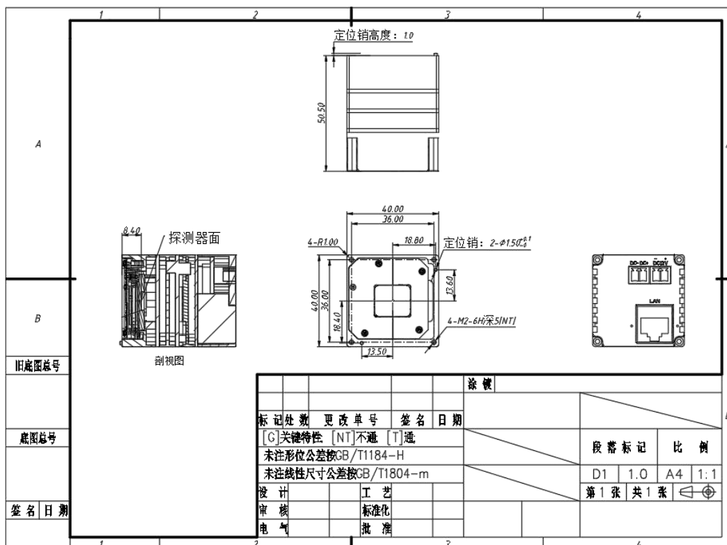
Figure 4 K26 movement structure dimensions
