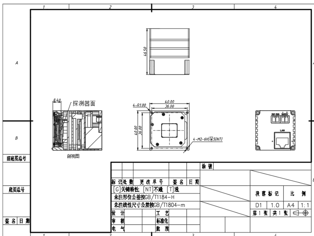
Figure 3 K23 movement structure dimensions
