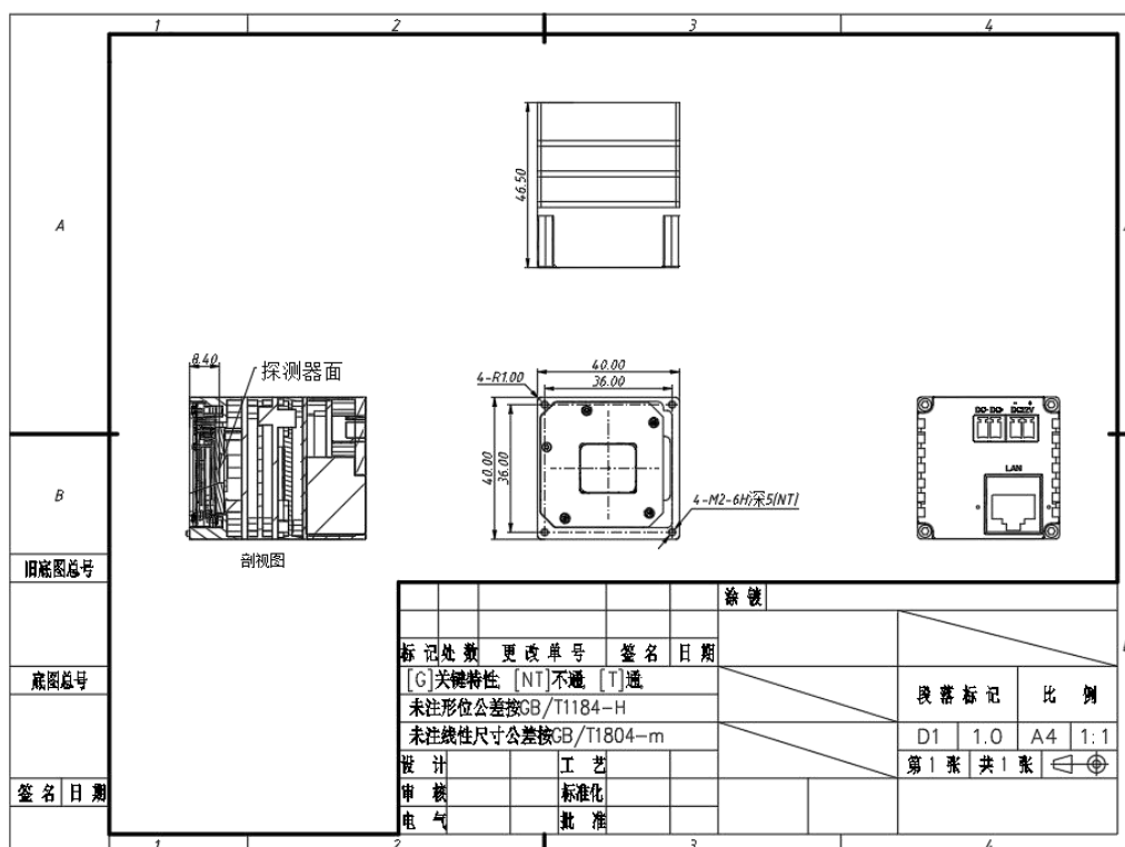
Figure 3 K23 movement structure dimensions
