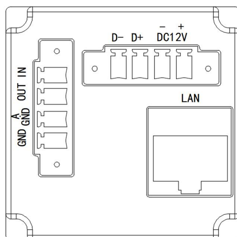
Figure 2 Interface board connector definition
